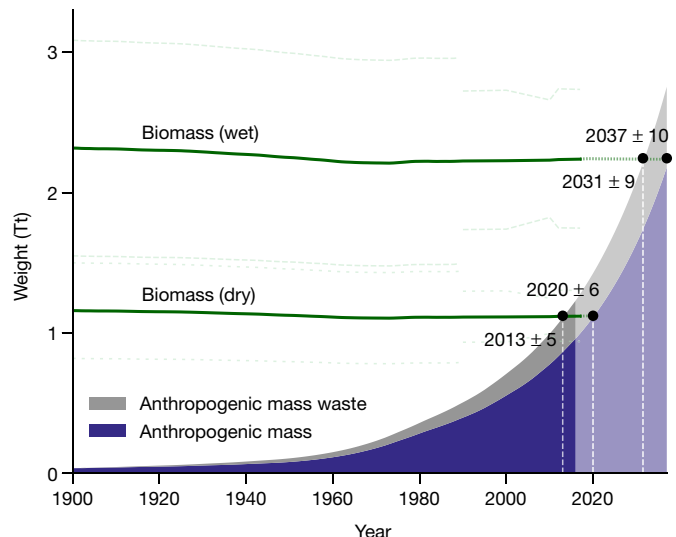
Fig. 2 | Biomass (dry and wet), anthropogenic mass and anthropogenic mass waste estimates since the beginning of the twentieth century. Green lines show the total weight of biomass ( \pm 1 s.d.). Anthropogenic mass weight is plotted as an area chart. The wet-weight estimate is based on the results presented in Fig. 1 and the respective water content of major components (see Methods). The year 2013 \pm 5 marks the time at which the dry biomass is exceeded by the anthropogenic mass, including waste. The years 2037 \pm 10 and 2031 \pm 9 mark the times at which the wet biomass is exceeded by the anthropogenic mass and the total produced anthropogenic mass, respectively. The uncertainties of the years of intersection were derived using a Monte Carlo simulation, with 10,000 repeats (see Methods). Weights are extrapolated for the years 2015–2037 (lighter area; see Methods).
