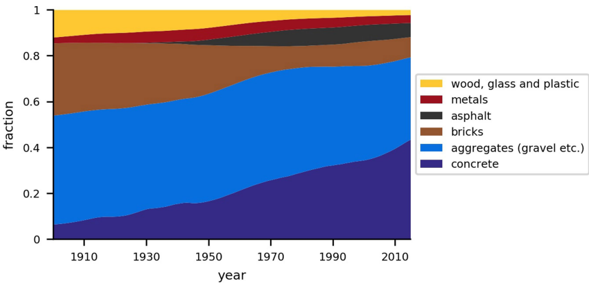
Extended Data Fig. 2 | Anthropogenic mass composition since the year 1900, divided into material groups. Dataset is based on ref. 22 .
