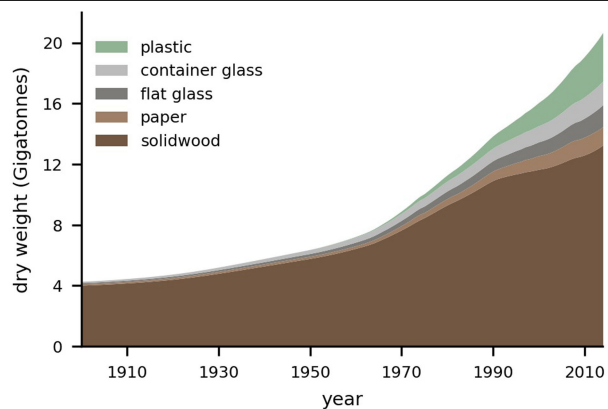
Extended Data Fig. 5 | Anthropogenic mass estimates for (industrial round) wood, glass and plastic since the beginning of the twentieth century, divided into material sub-groups. Data are taken from the comprehensive work of the Institute of Social Ecology, Vienna. We used a recent study 71 , which has some minor updates compared to the study used to achieve the main results 22 .
